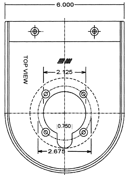
8320 - Gas Spill Tray, No Vent (Black)
