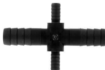
3701 - NEW 5/8" Barb, 5/16" Barb, 5/8" Barb, 5/16" Barb
