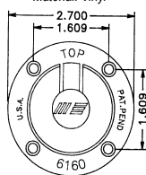
6160 - 2.7" One-Piece Rubber Scupper with Flap (Black)
