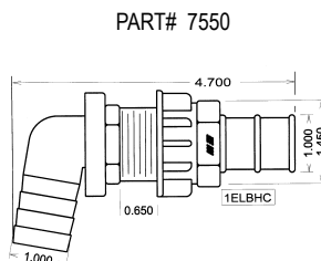
1" Elbow Bulkhead Connector
