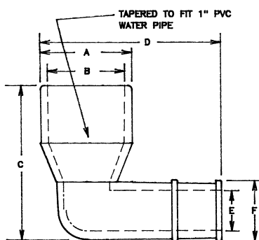
9095 - 1 1/8" Overflow Elbow
