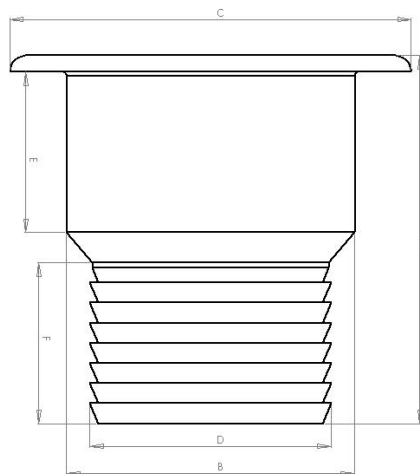
7182 - NEW 3" Scupper with Long Thread
