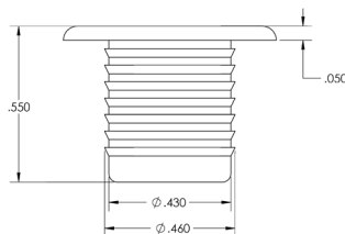
Marine East Part - 6229 / 6229W Impact LED Holder. * For Reference Only *
