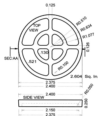
8390 - 2" Elbow Screen (Black)
