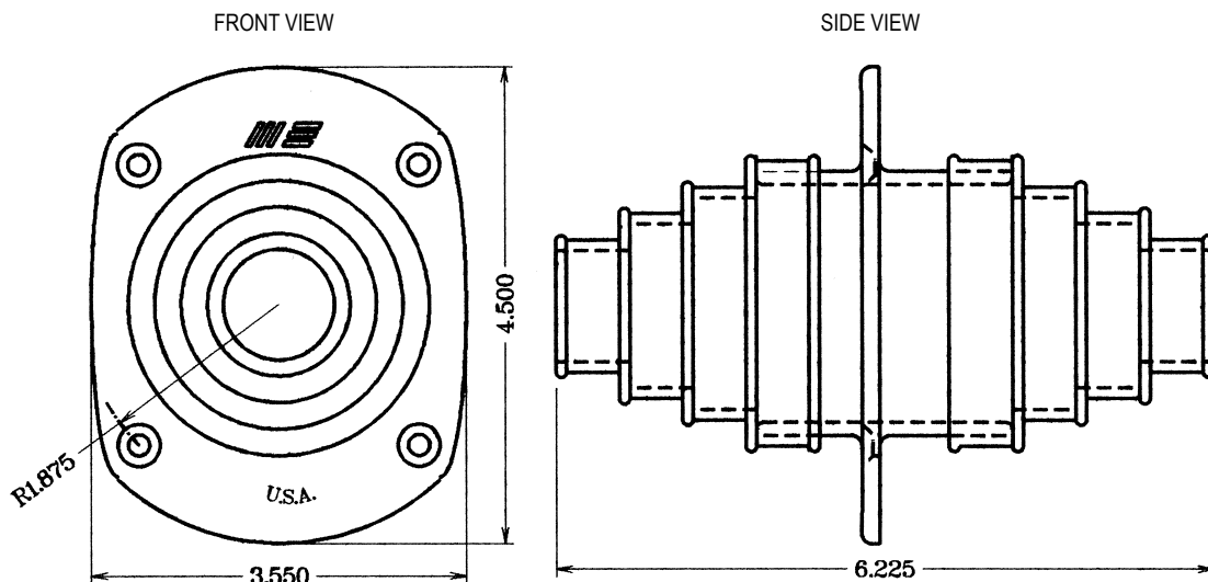
ASSEMBLED BULKHEAD FITTING WITH END COVERS ATTACHED
