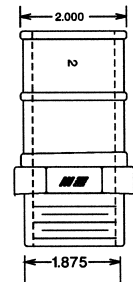
PART # 8496ST 2" BARB 1 1/2" STRAIGHT MPT
