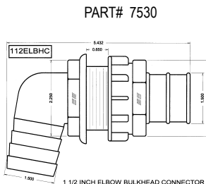
1 1/2" Elbow Bulkhead Connector
