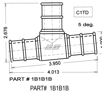
1B1B1B - 1" Barb, 1" Barb, 1" Barb
