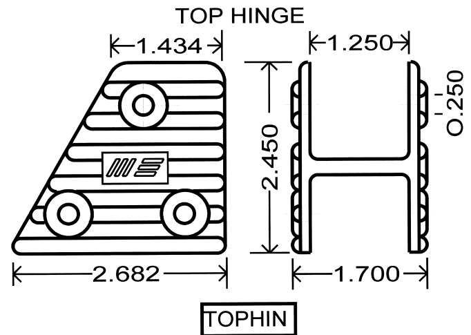
4570G - Top Mount Swivel Hinge (Gray)
