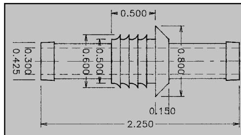
Shielded Barb-to-Barb Impact Drain
