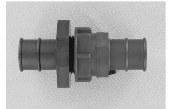
7951 - 1 1/8" Compact Bulk Head Assembly
