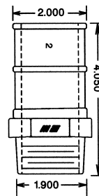
PART # 8484 2" BARB 2" TFPT
