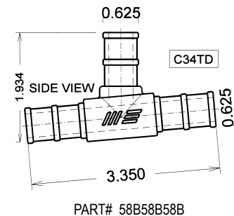
58B58B58B - 5/8" Barb, 5/8" Barb, 5/8" Barb
