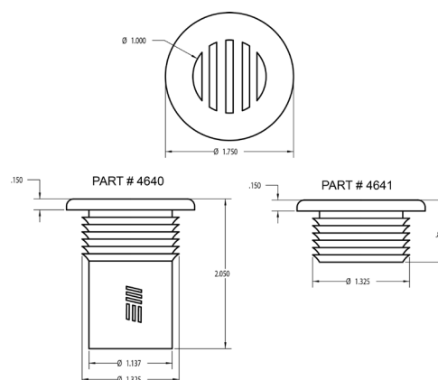
4640 - 1 1/8" Impact Vent, Long & 4641 - 1 1/8" Impact Vent, Short (Top)
