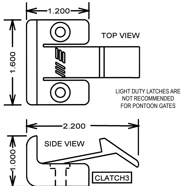
4046 - Light Duty Latch
