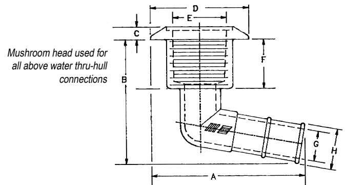
6300W - 1 1/8" Mushroom Head Thru-Hull (White)
