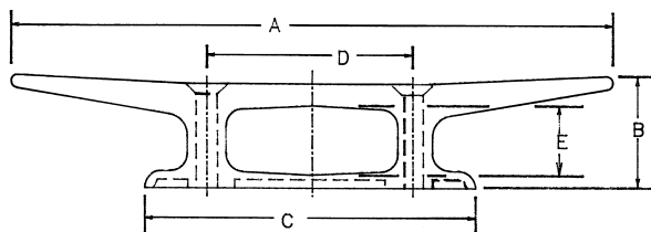
2101, 2103, and 2105 - 4", 6", and 8" Cleats
