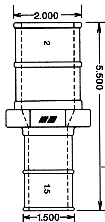
PART # 8495 2" BARB 1 1/2" BARB
