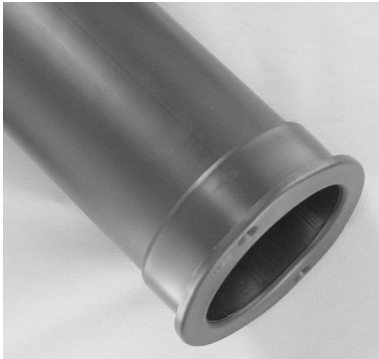
6673 - 3" Diameter, 4' Rod Holder Tube with Trapezoidal Trim Ring
