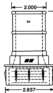
PART # 8484 2" BARB 2" TFPT
