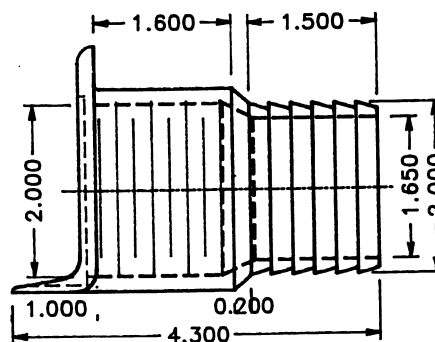
6118W - 2" Barbed End Scupper with Inner Crosshairs
