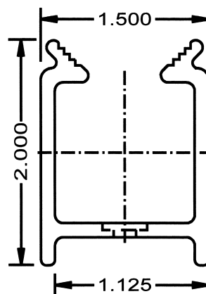
4415 - 1 1/4" Square Tubing Clip w/ Guide (Black)
