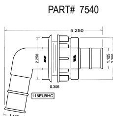
1 1/8" Elbow Bulkhead Connector
