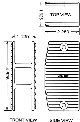
4028 Extra Long Pontoon Boat Sliding Bimini Hinge (Black)
