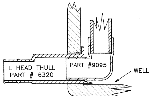
Above: 9145 - 1 1/2" T" Drain, 16 1/2" Tube
