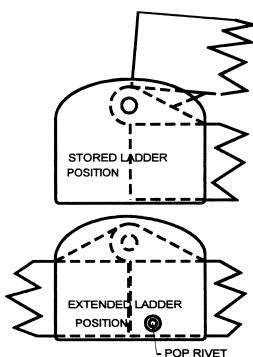
4365 - Rectangular 1" x 2" Ladder Guard
