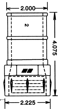
PART # 8494 2" BARB 1 1/2" FPT
