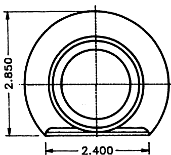
6103W - Full Thread with Flap
