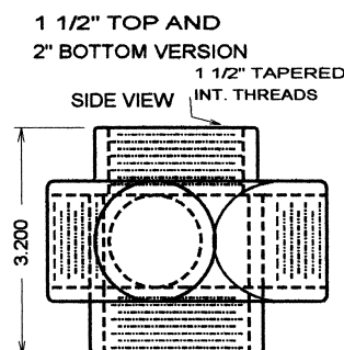
1610 - 1 1/2" Top Thread, 2" Bottom Thread Manifold (Black)
