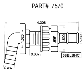
5/8" Elbow Bulkhead Connector
