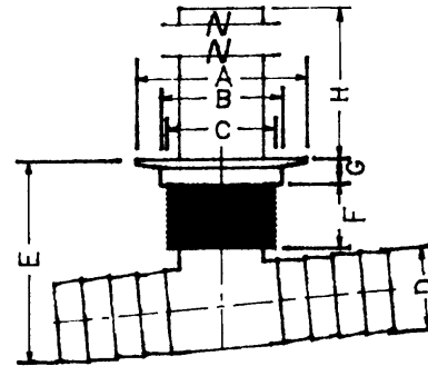
4121C - 1 1/2" w/Crosshairs (chrome)
