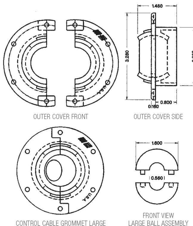
1840W - Control Cable Grommet (White)
