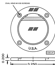
6170 - Scupper Back Down Valve Assembly
